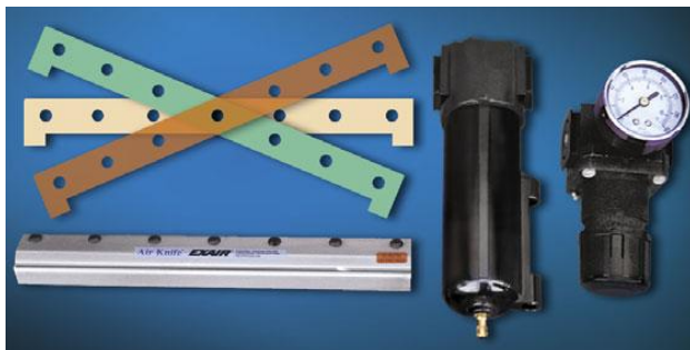
Kits include a Standard Air Knife, shim set, filter separator, and pressure regulator (with coupler).
